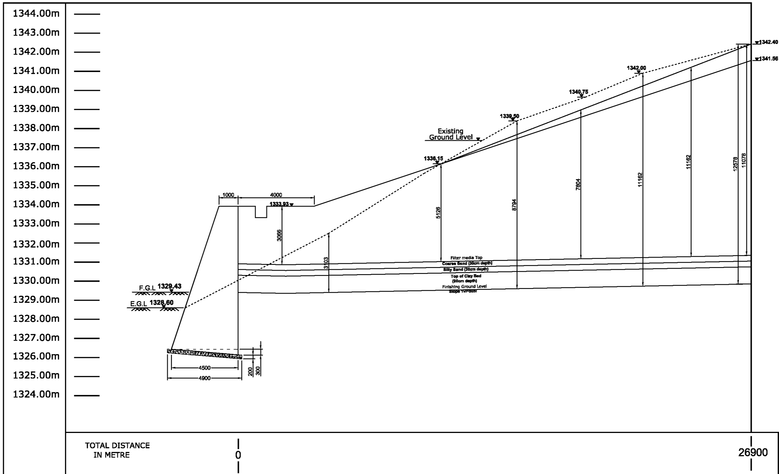
Cross Section at A2-A2-1
