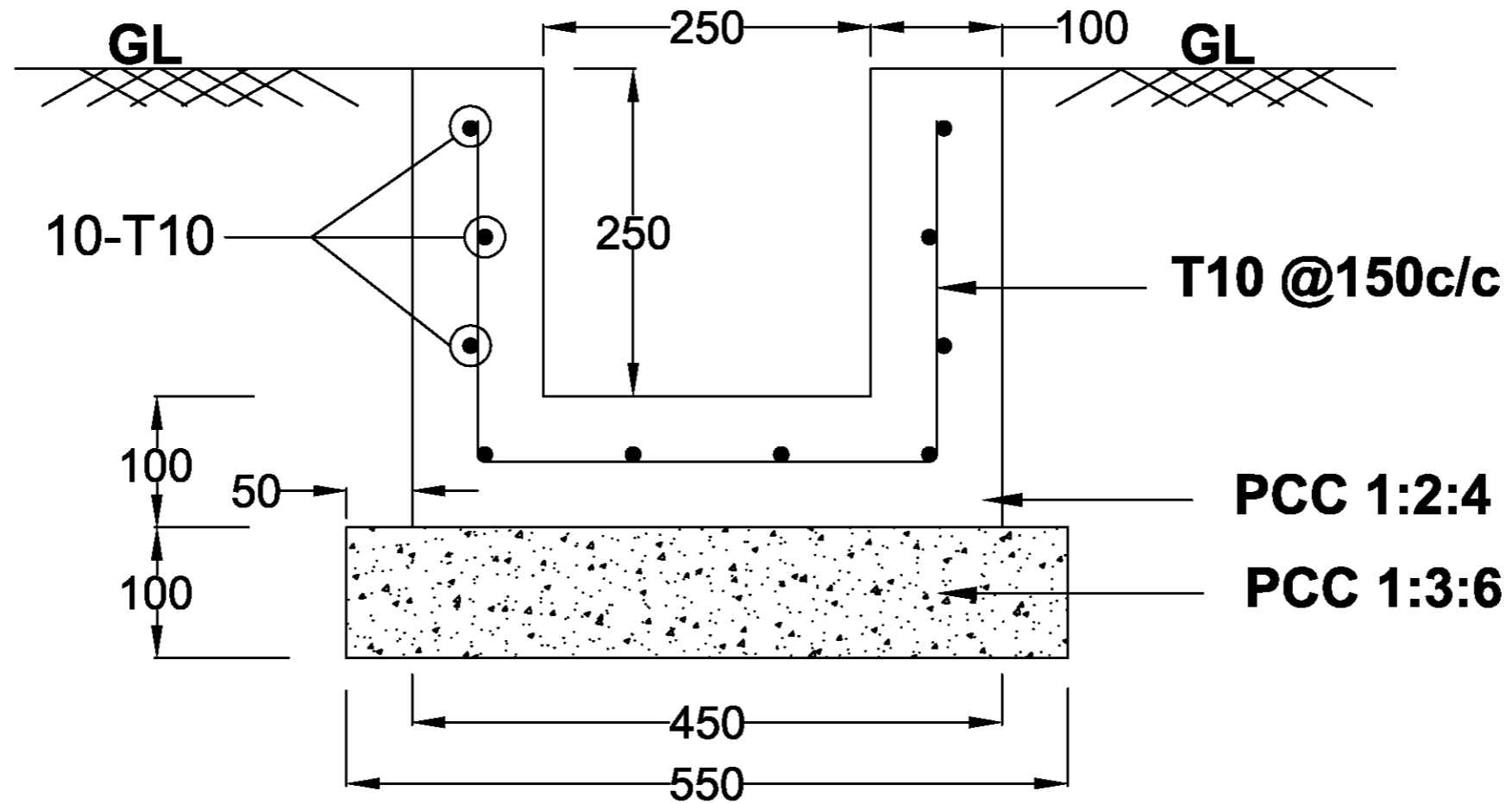
Cross Section of Open Drain 250x250
