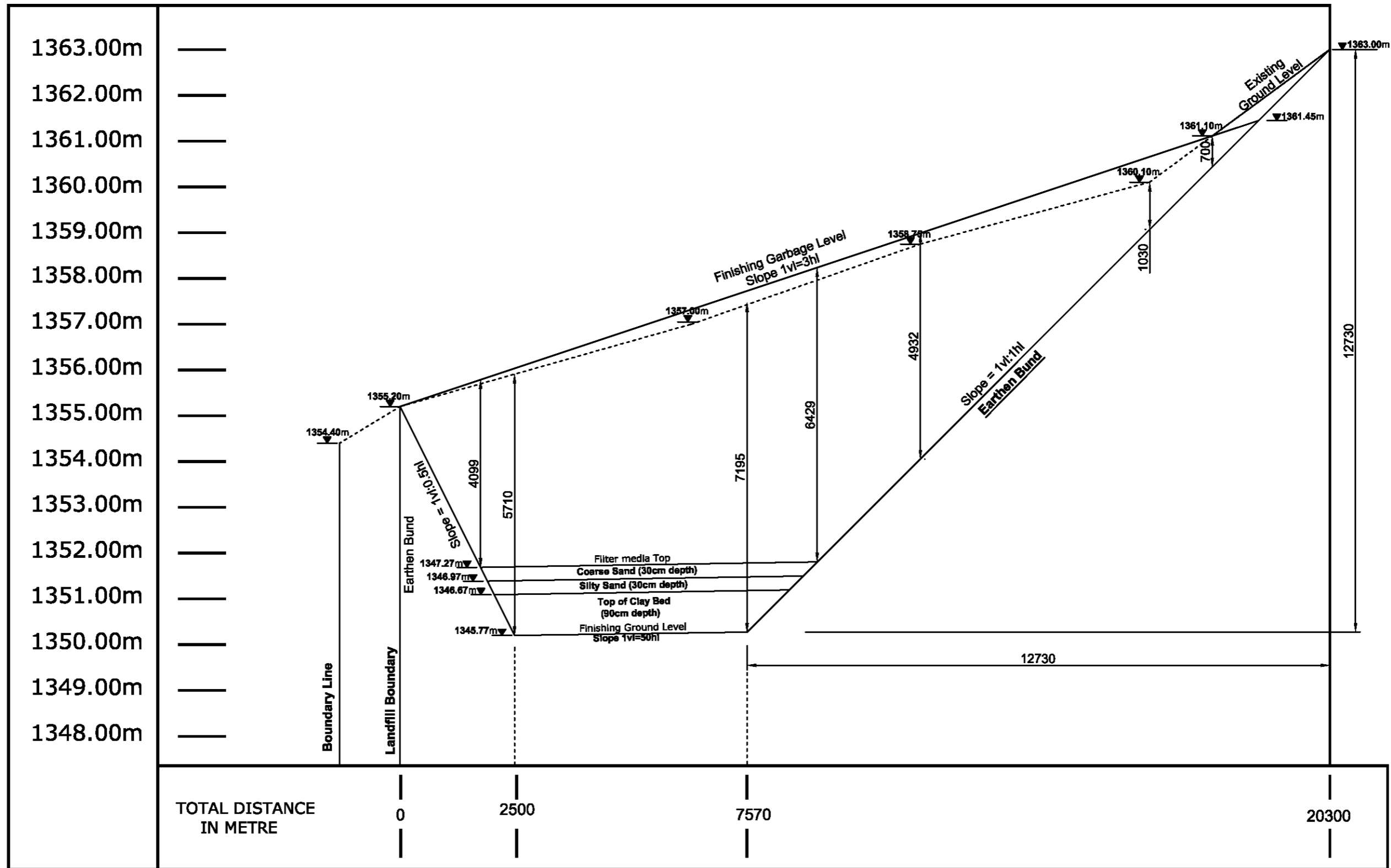
Cross Section at A15-A17
