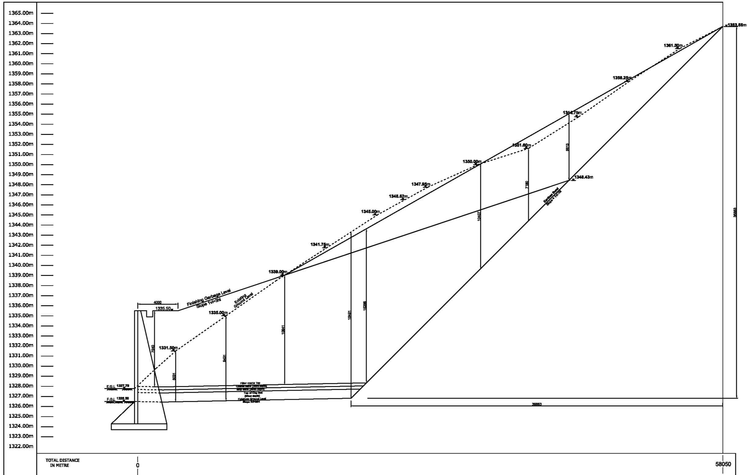
Cross Section at A11-A19
