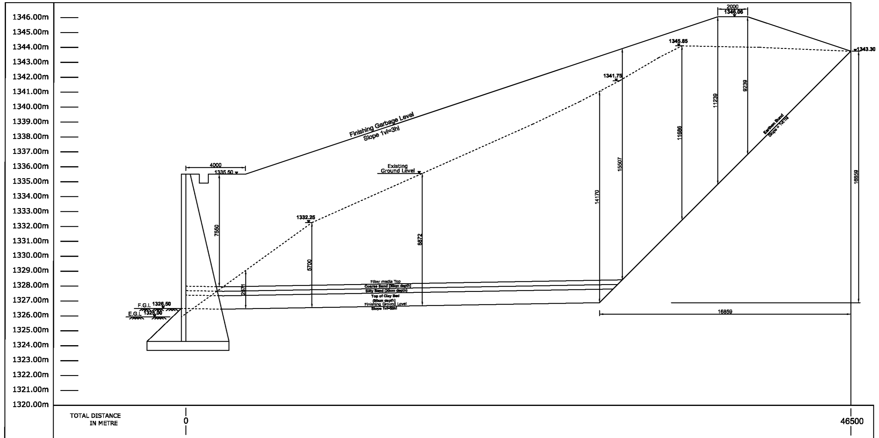
Cross Section at A7-A24
