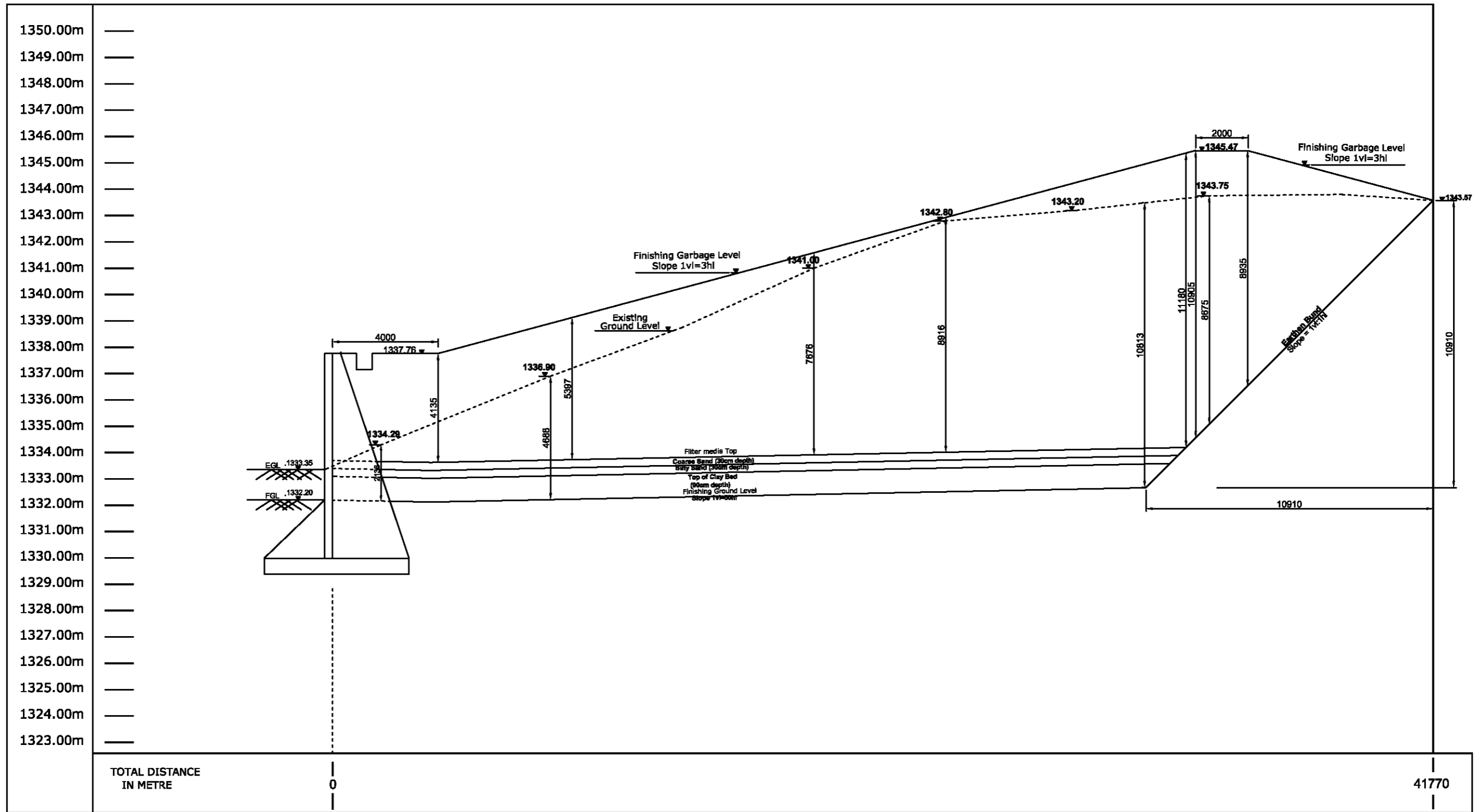
Cross Section at A5-A26
