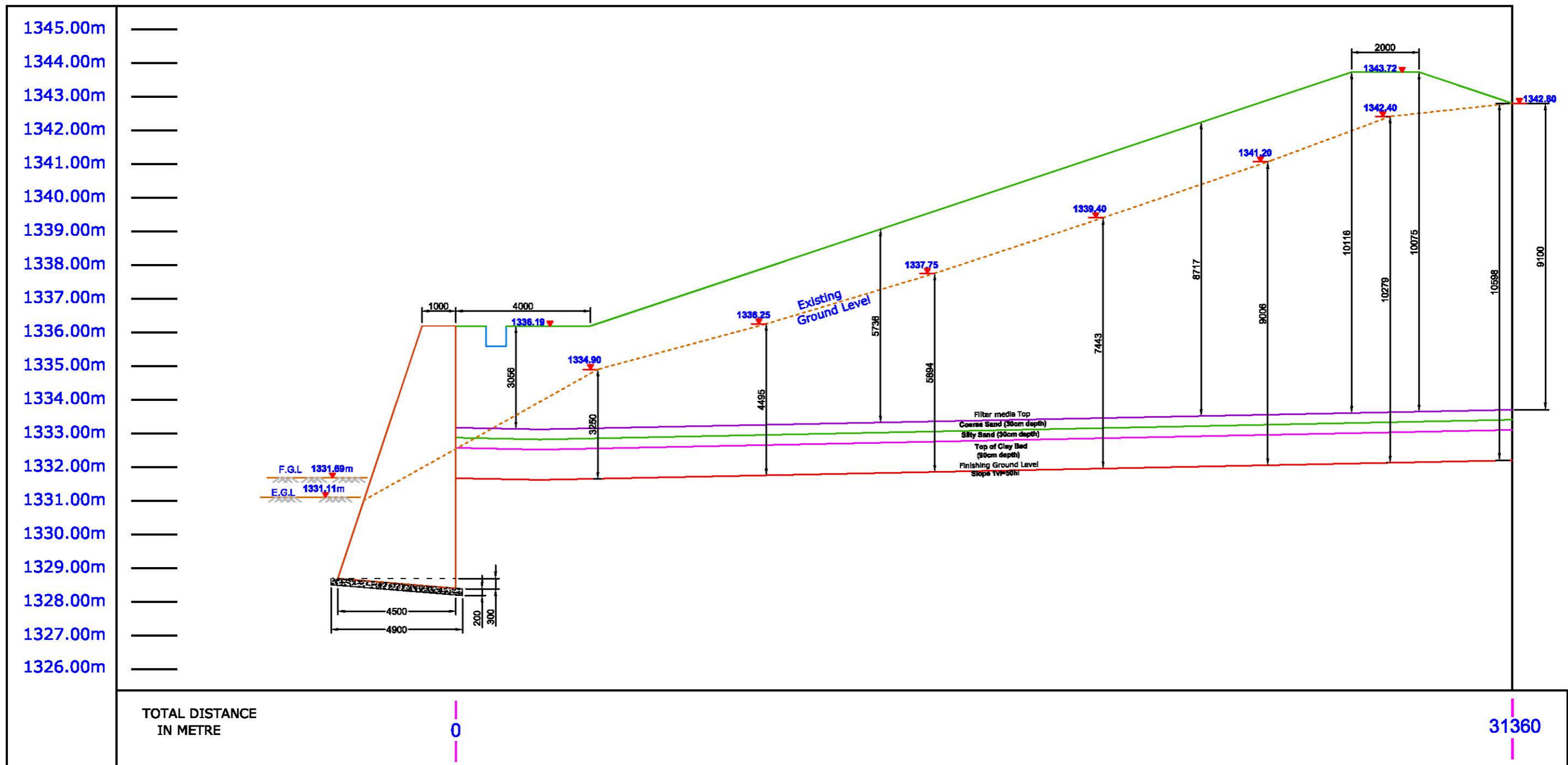
Cross Section at A3-A3-1
