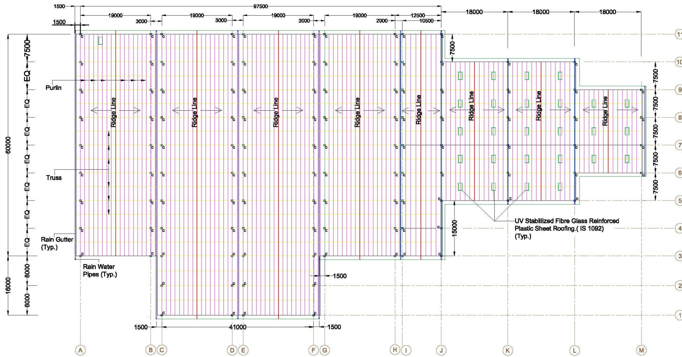
Truss Roof Plan
