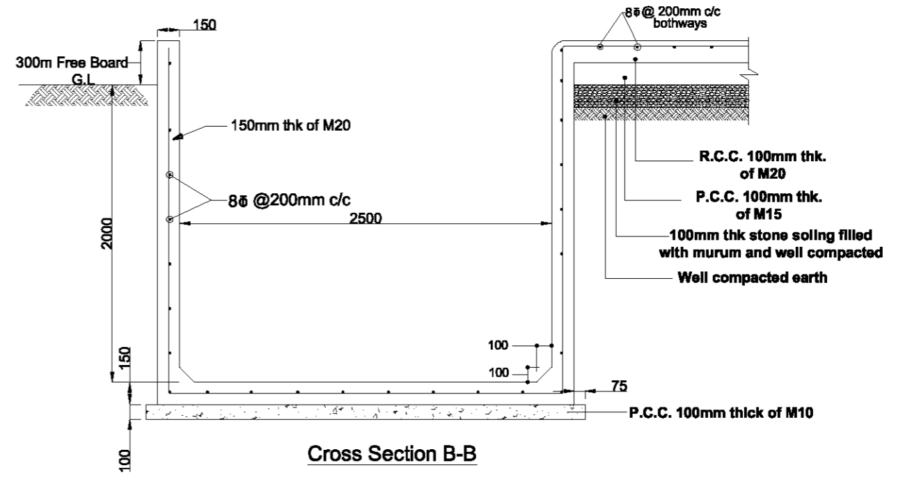
Leachate Holding Tank
