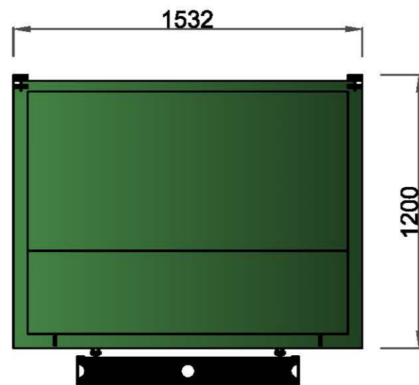
BACK SIDE VIEW GARBAGE TIPPER VEHICLE (2.0 CUM CAPACITY)
