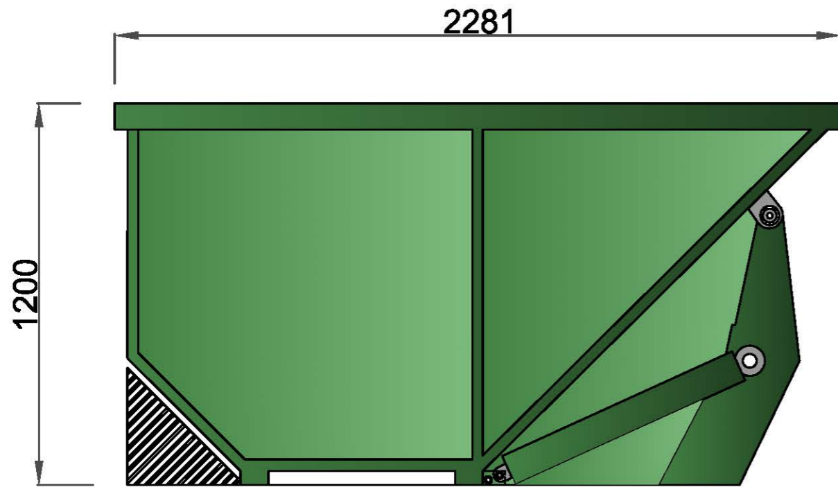
SIDE VIEW GARBAGE TIPPER VEHICLE (2.0 CUM CAPACITY)
