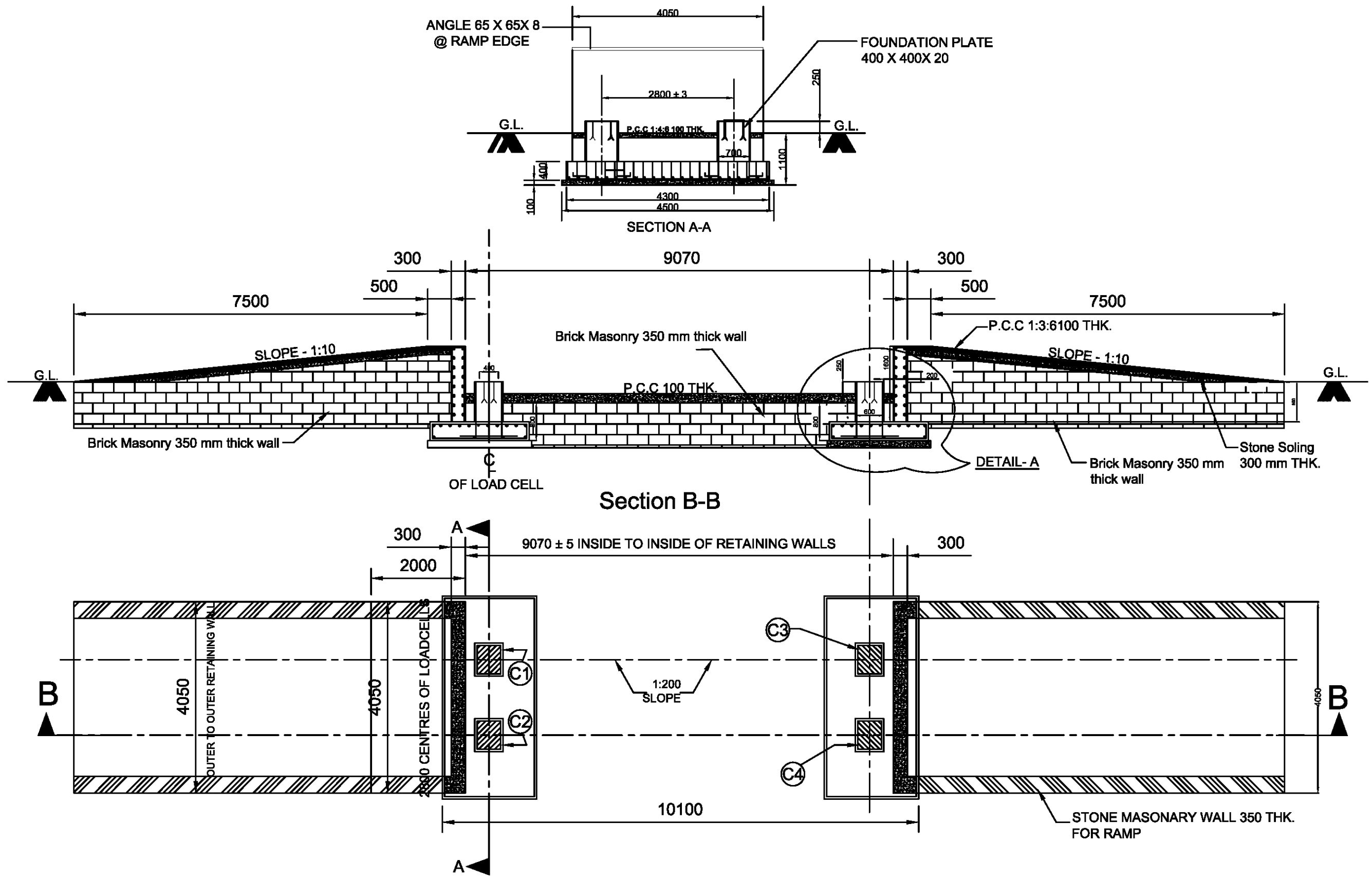
PLAN OF COLUMNS / FOOTINGS / RETAINING WALL OF TRUCK SCALE
