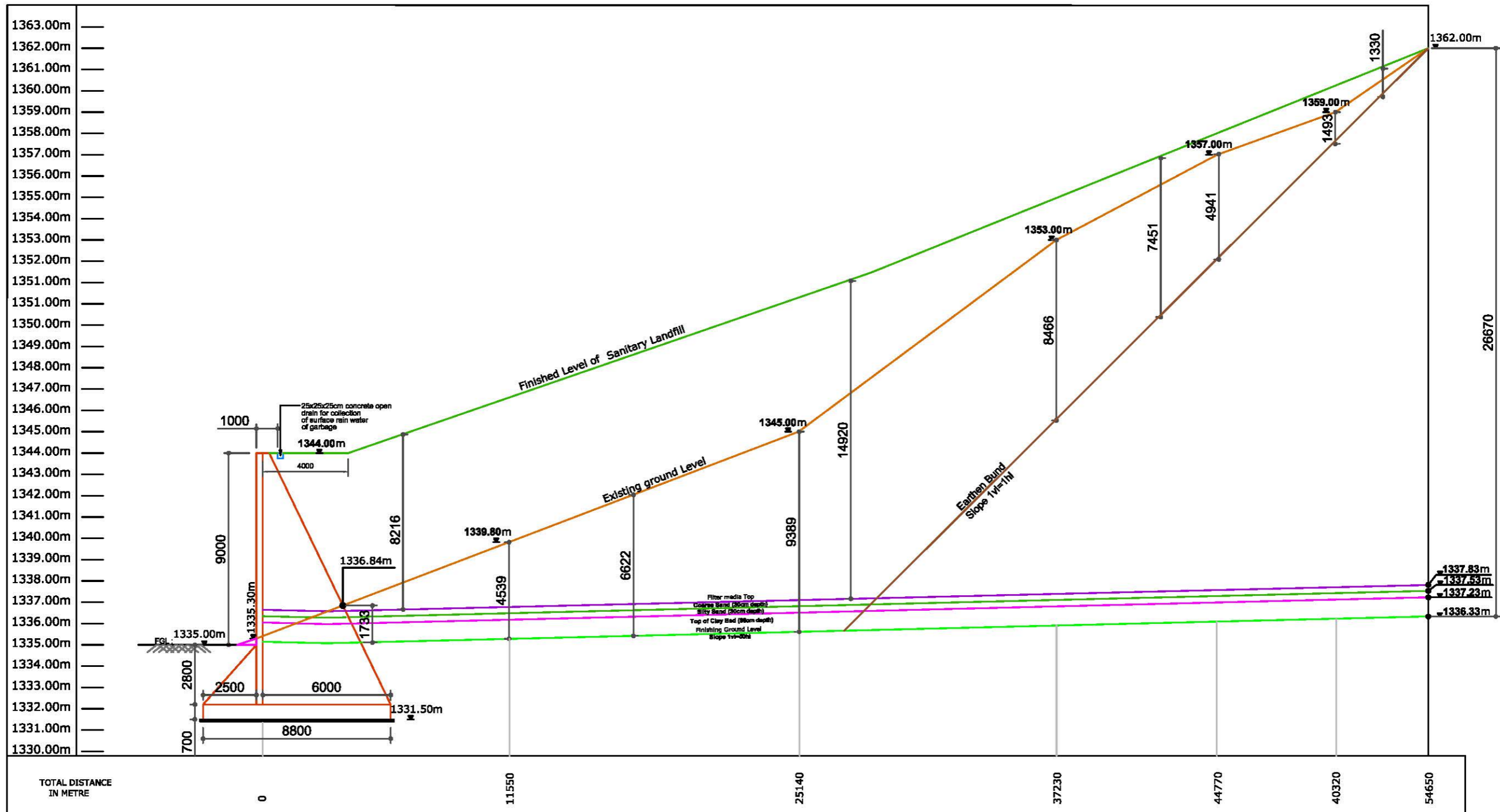
Cross Section at J-U of Proposed Landfill
