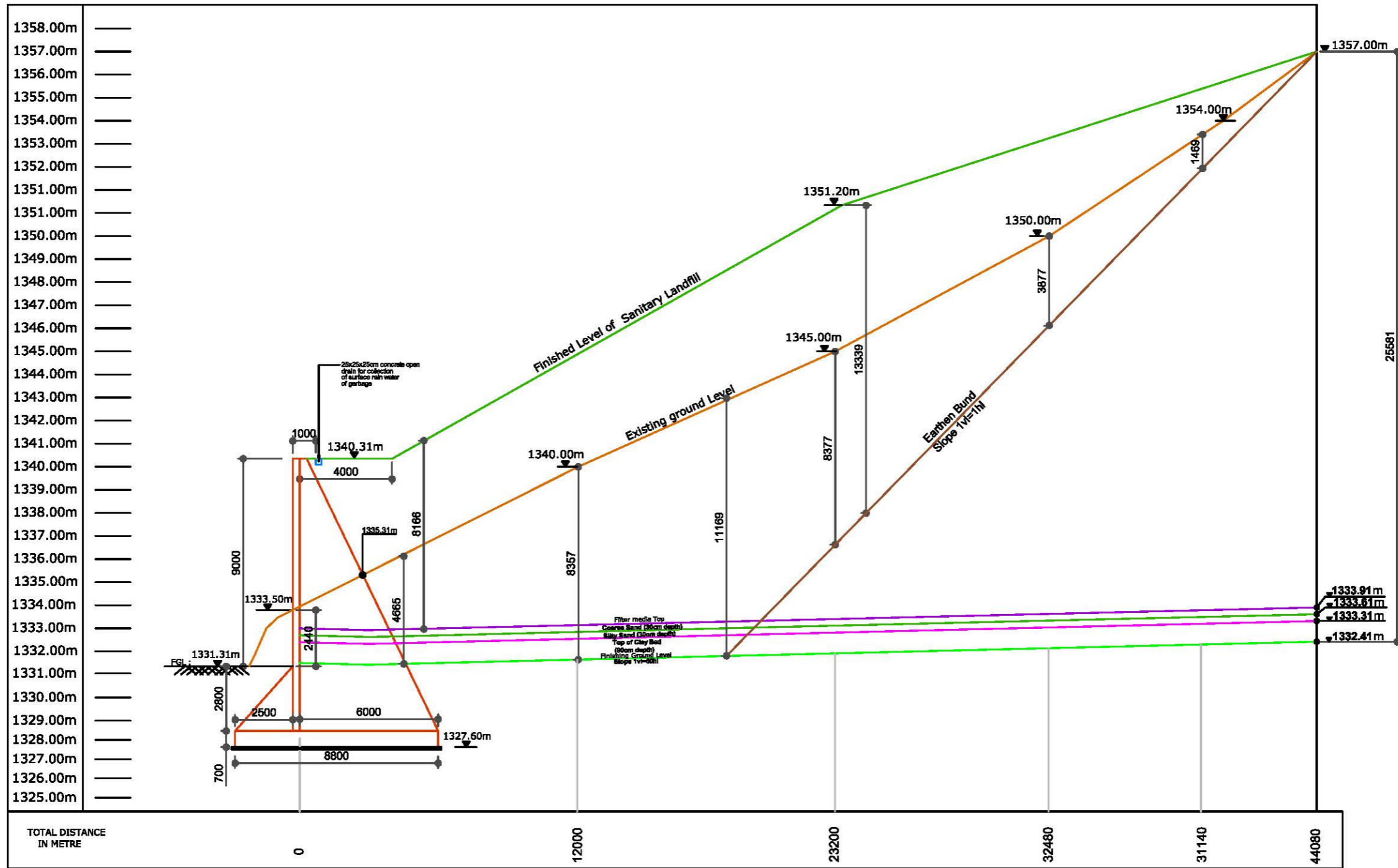
Cross Section at A1-A2 of Proposed Landfill
