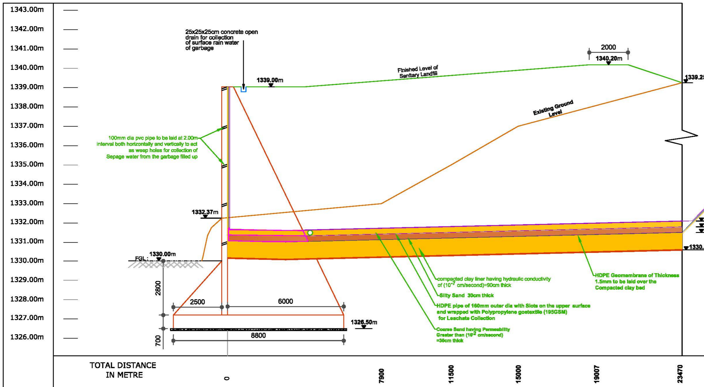
Typical Cross Section of Proposed Landfill
