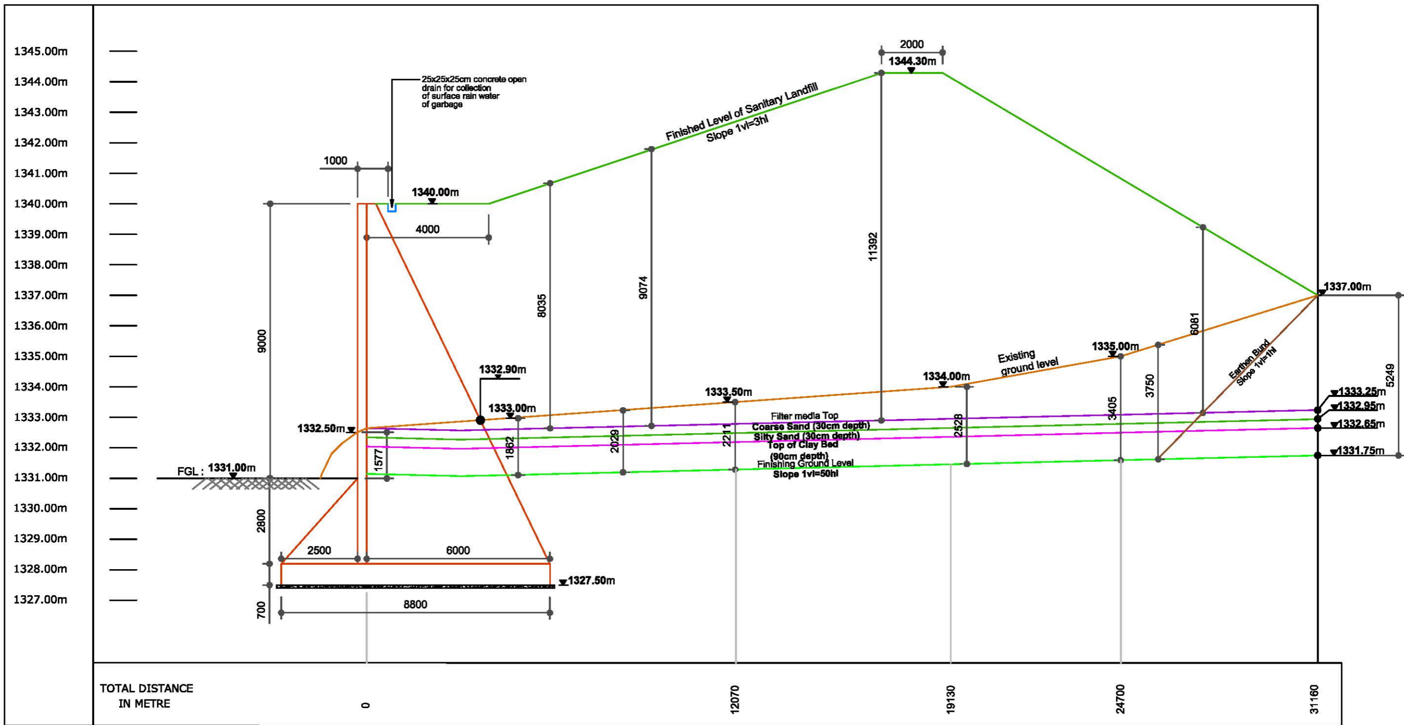
Cross Section at D-Z of Proposed Landfill
