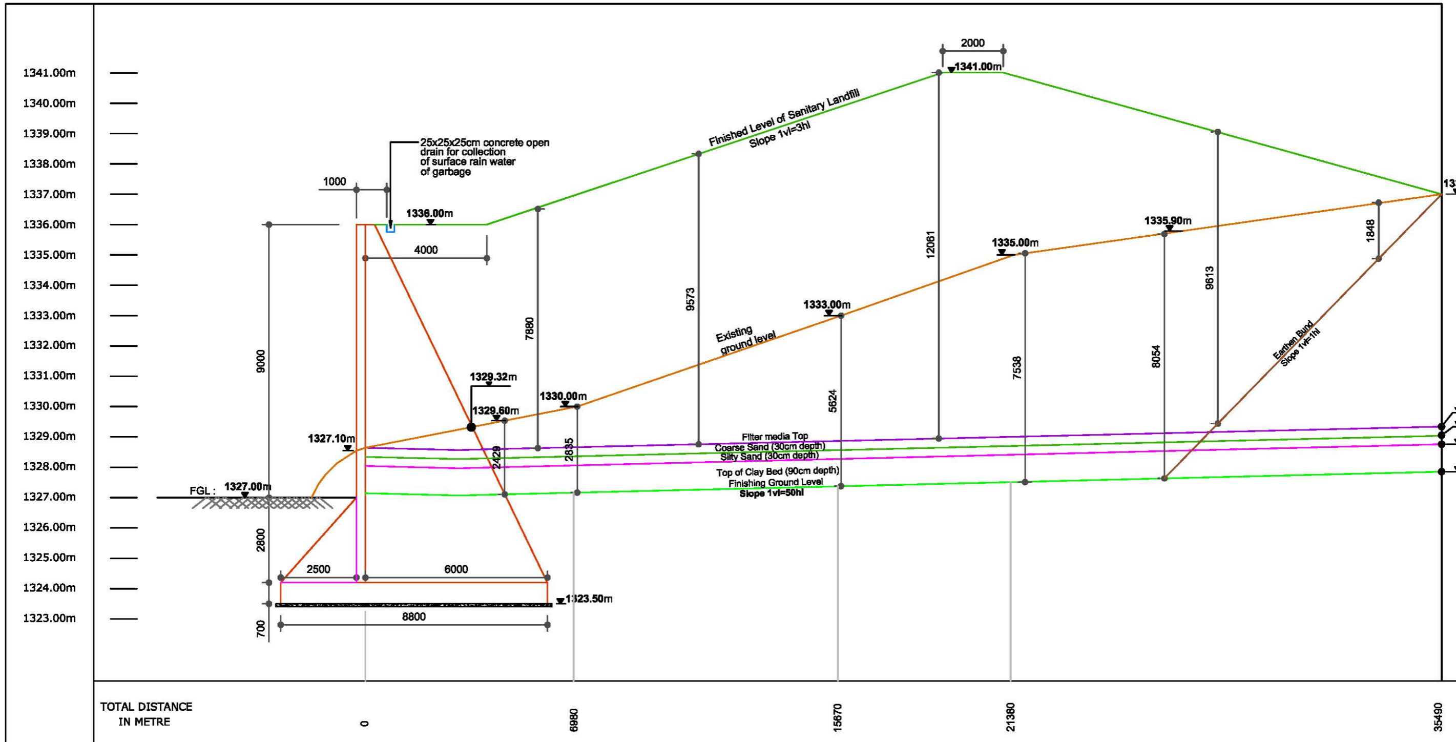
Cross Section at E-Z of Proposed Landfill
