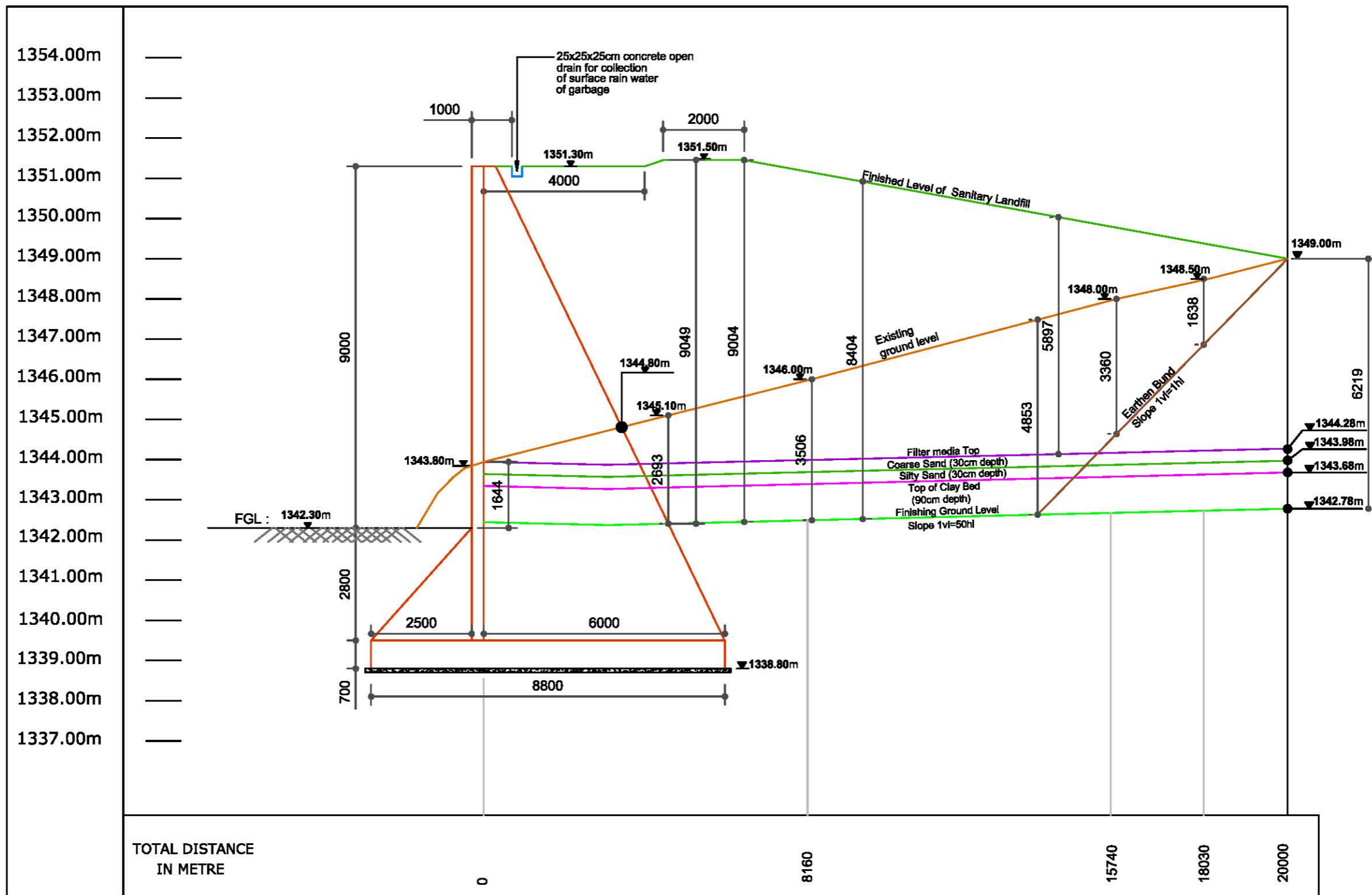
Cross Section at N-Q of Proposed Landfill
