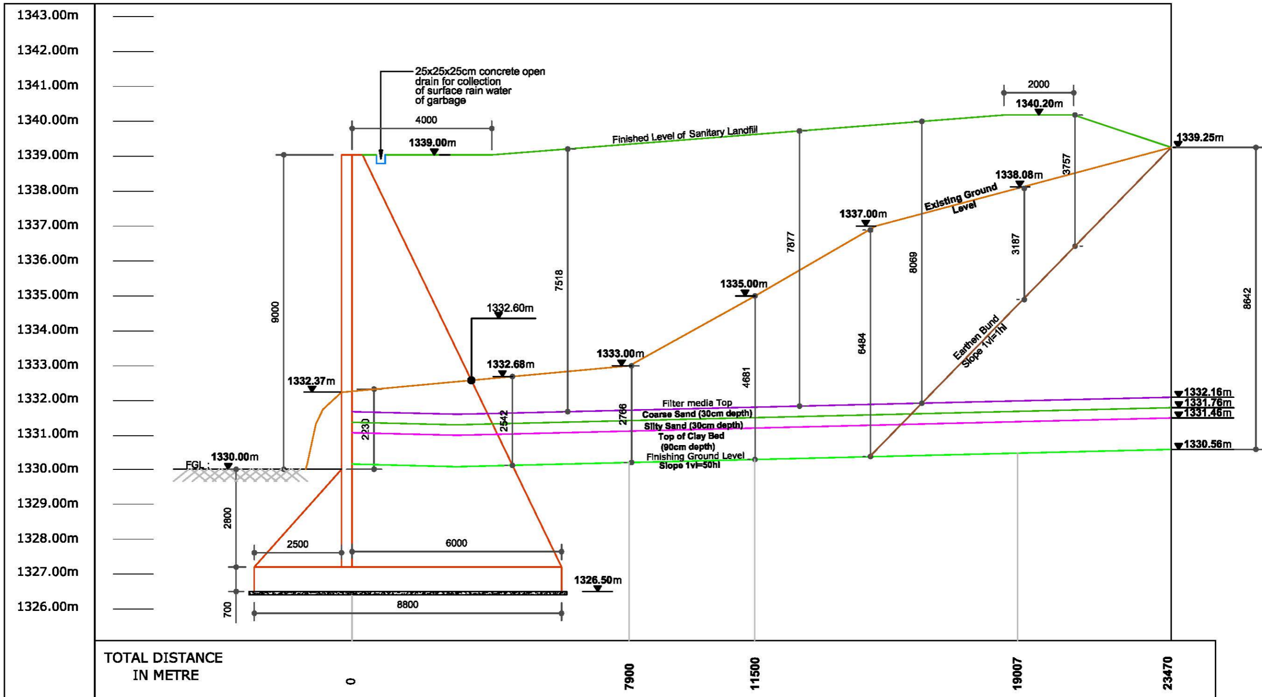
Cross Section at H-X of Proposed Landfill
